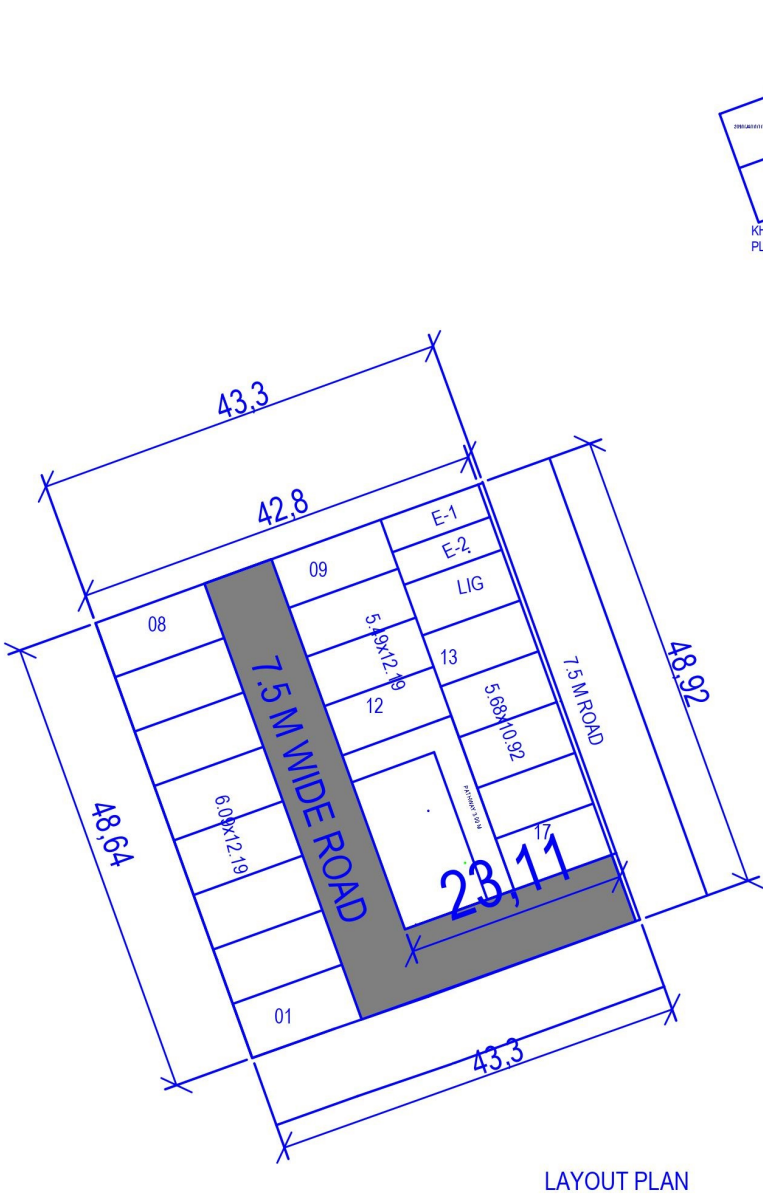
LAYOUT PLAN
