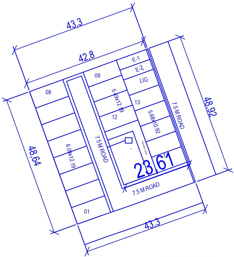
LAYOUT PLAN
